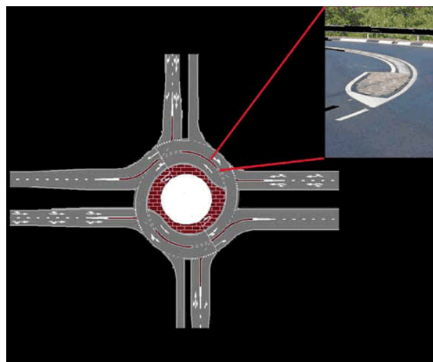
Figure 4 A “turbo” roundabout
